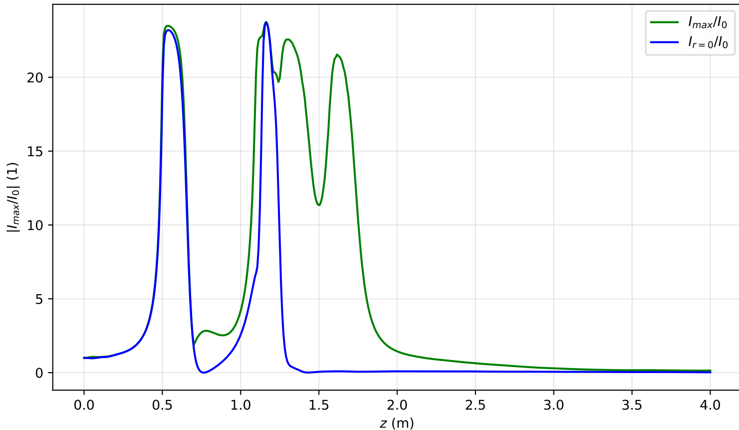
I_{max}(x = 0, y = 0, z)/I_0 , Pin=4.7Pcr, noisy input, artificial time
